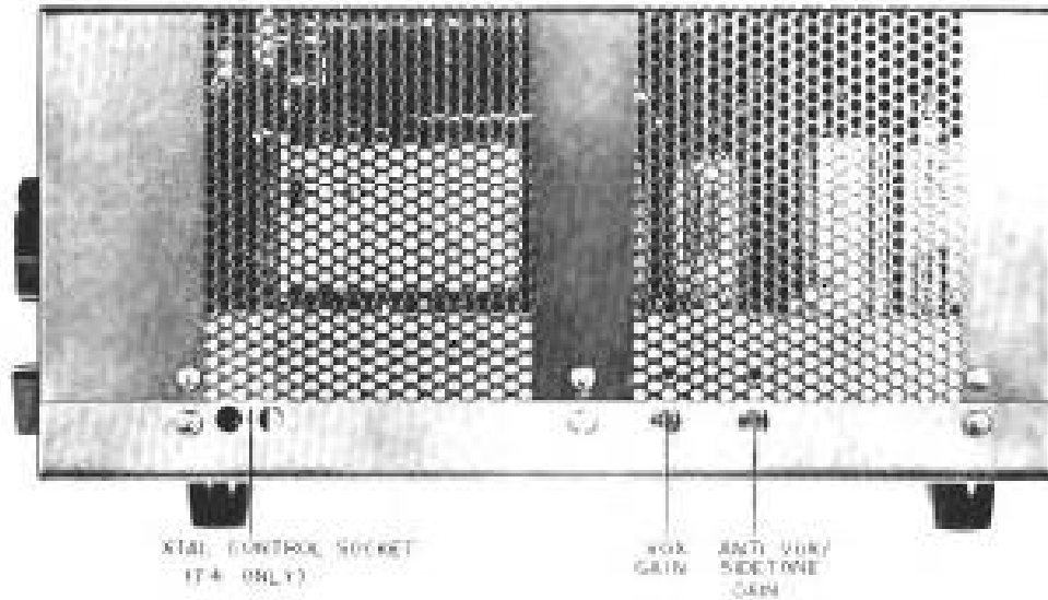
FIGURE 5 SIDE VIEW
