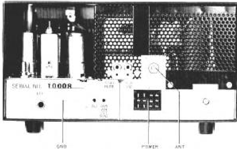
FIGURE 6 REAR VIEW
